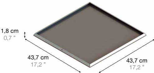
GRIDDLE / PLANCHA
